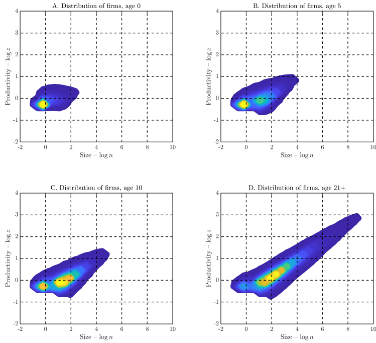
Figure 2: The model’s firm distribution in the space of productivity z and size n at different point of the life cycle.
