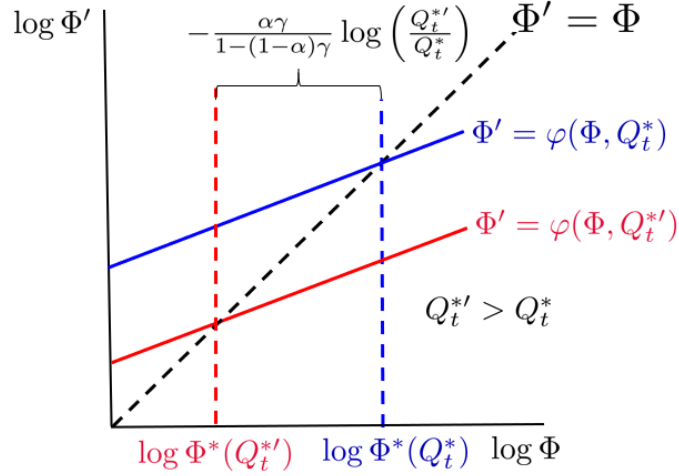
Figure 3: Macro of recruiting intensity decisions
