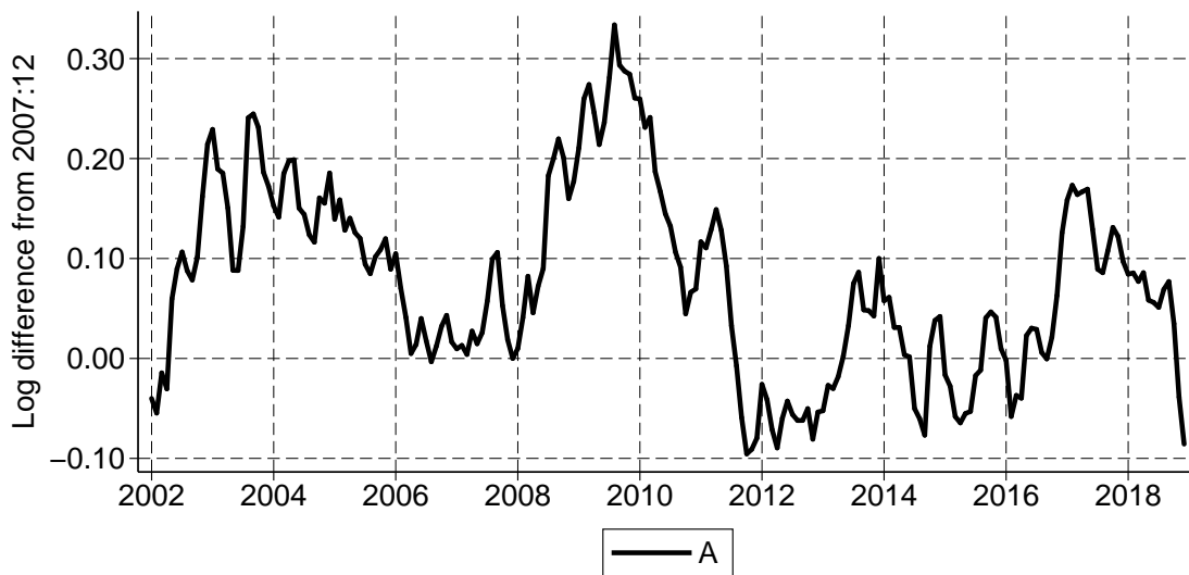
Figure A3: Residual match efficiency
